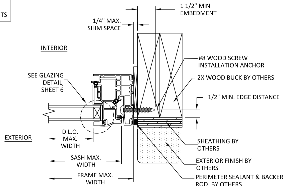
D 4 HORIZONTAL SECTION THROUGH FRAME INSTALLATION WOOD SUBSTRATE
